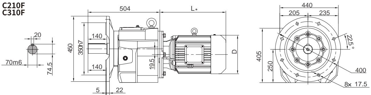
Flange-mounted
