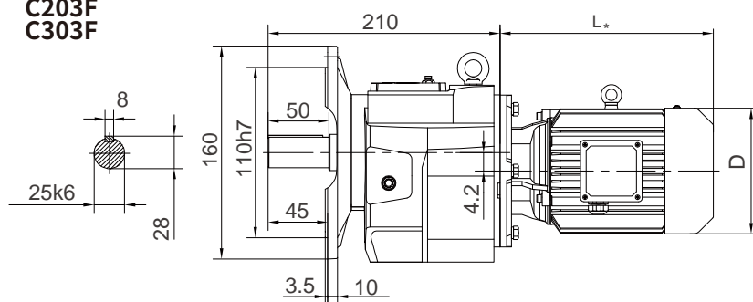
Flange-mounted
