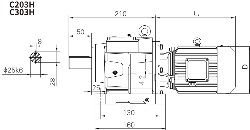
Horizontal foot-mounted
