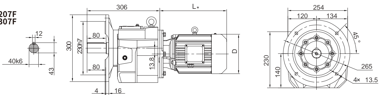
Flange - mounted
