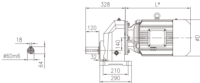
Horizontal foot-mounted
