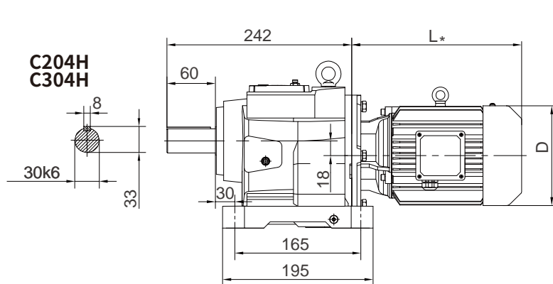
Horizontal foot-mounted
