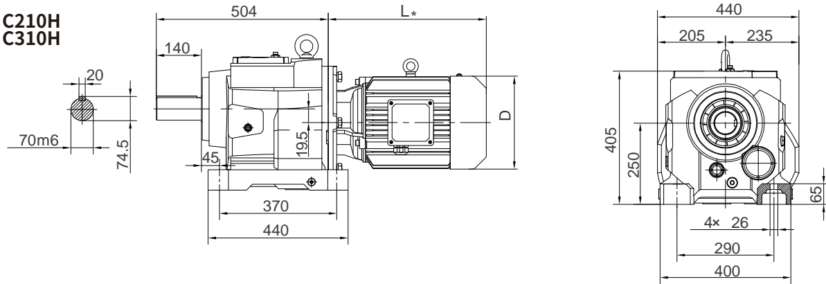
Horizontal foot-mounted
