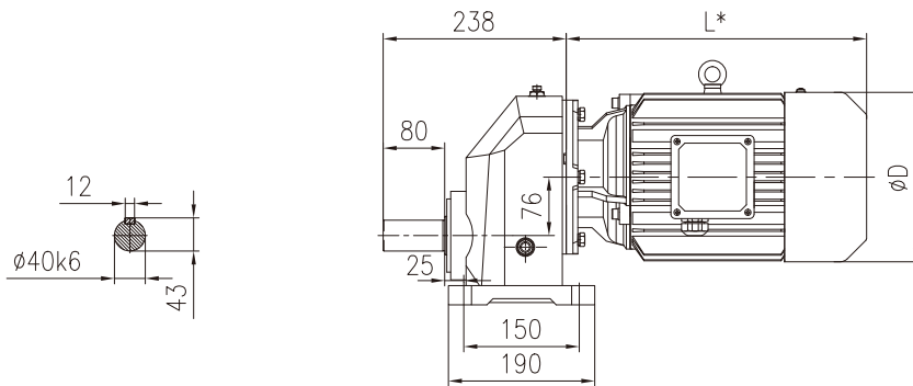
Horizontal foot-mounted
