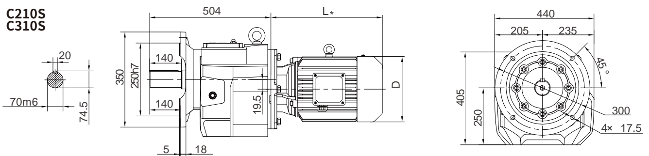
Short flange-mounted
