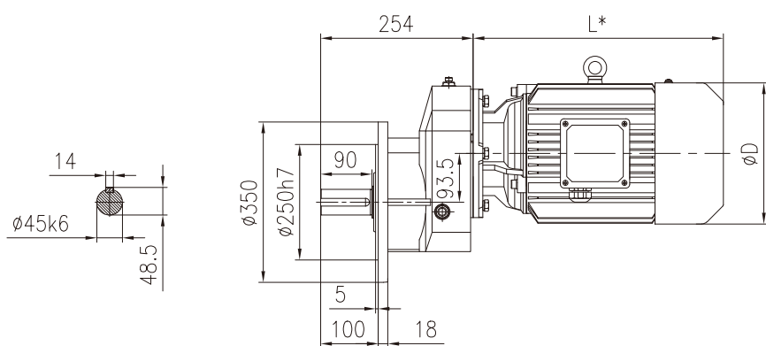
Flange - mounted
