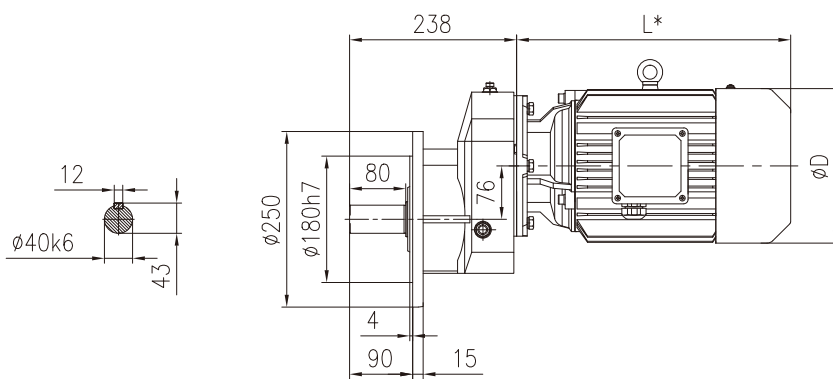
Flange - mounted
